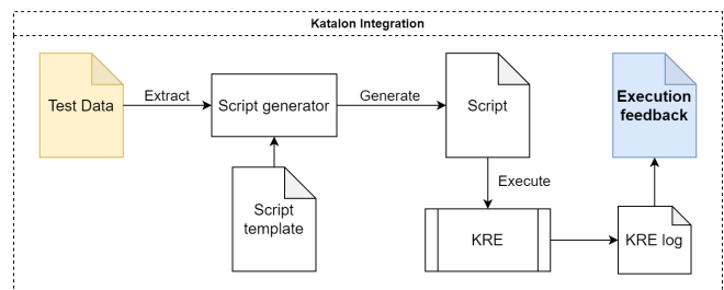
Figure 4: Katalon Integration
